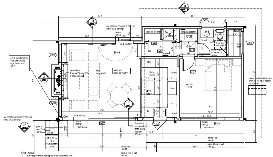
SENIOR UNIT FLOOR PLAN
