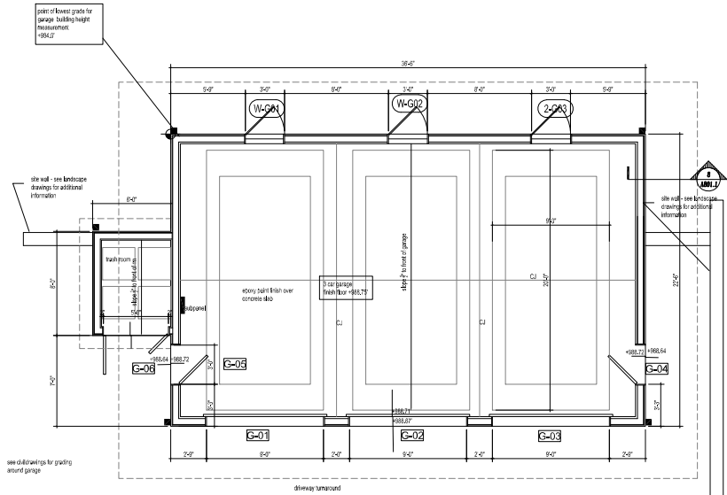
GARAGE FLOOR PLAN
